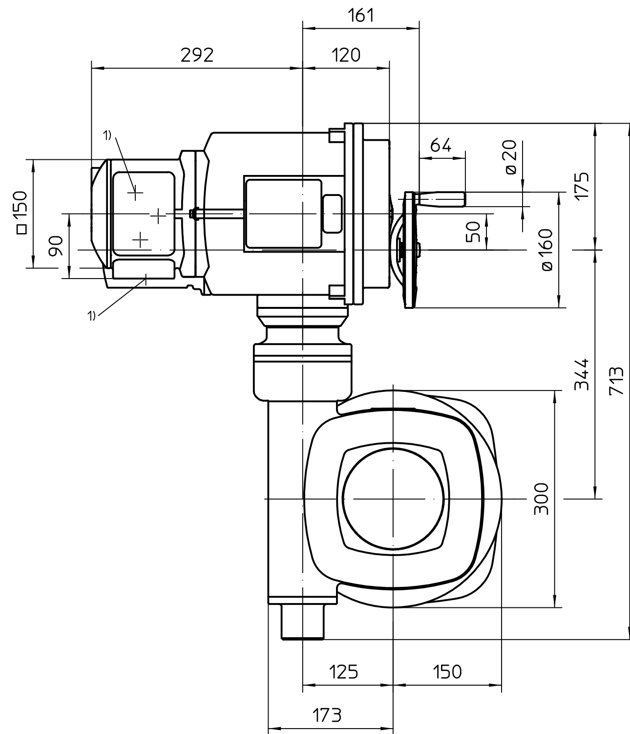
Standard Electrical connection in "Ex e" version
