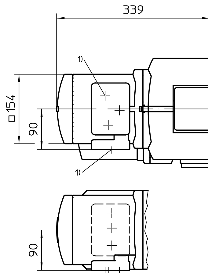
Option Electrical connection in "Ex d" version
