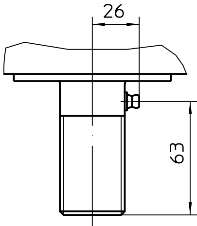
Detail X M 1:2
