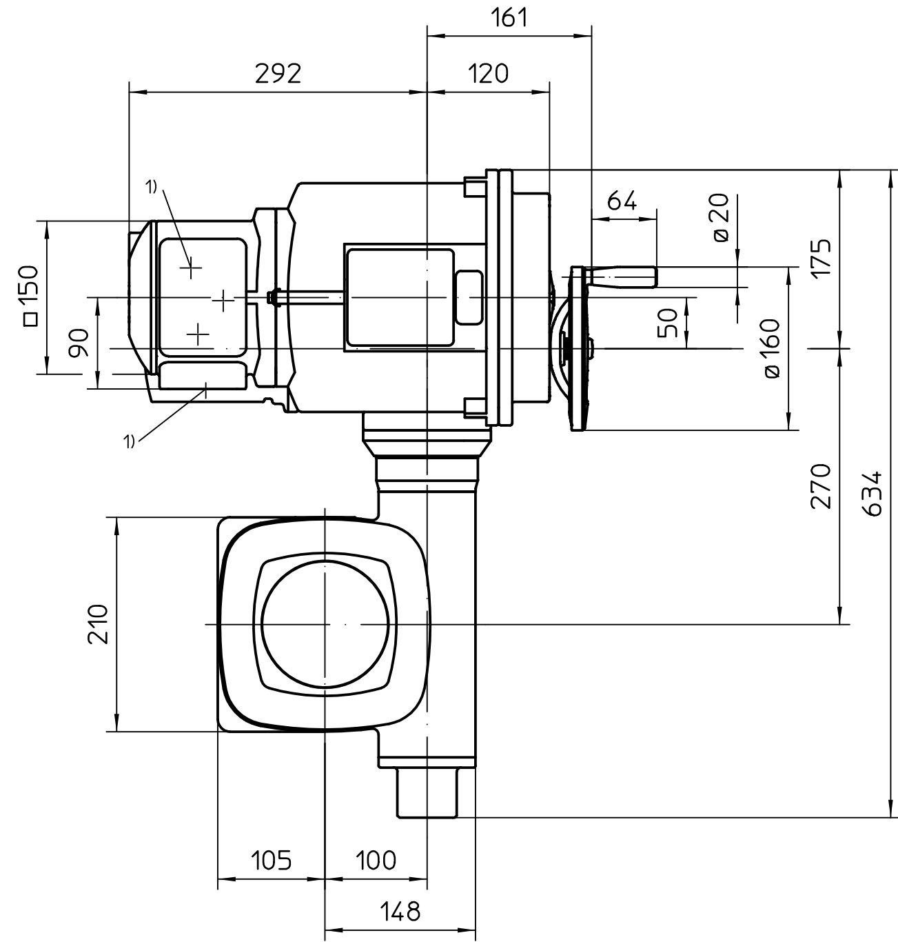
Standard Electrical connection in "Ex e" version
