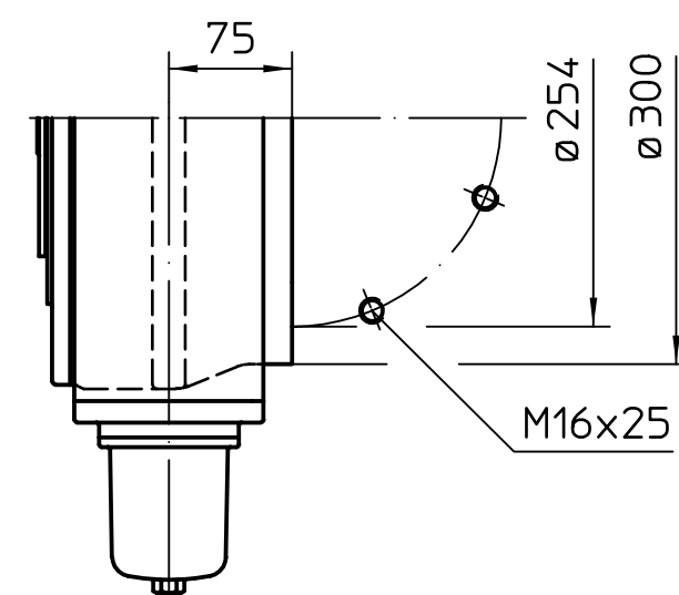
Plane flange option
