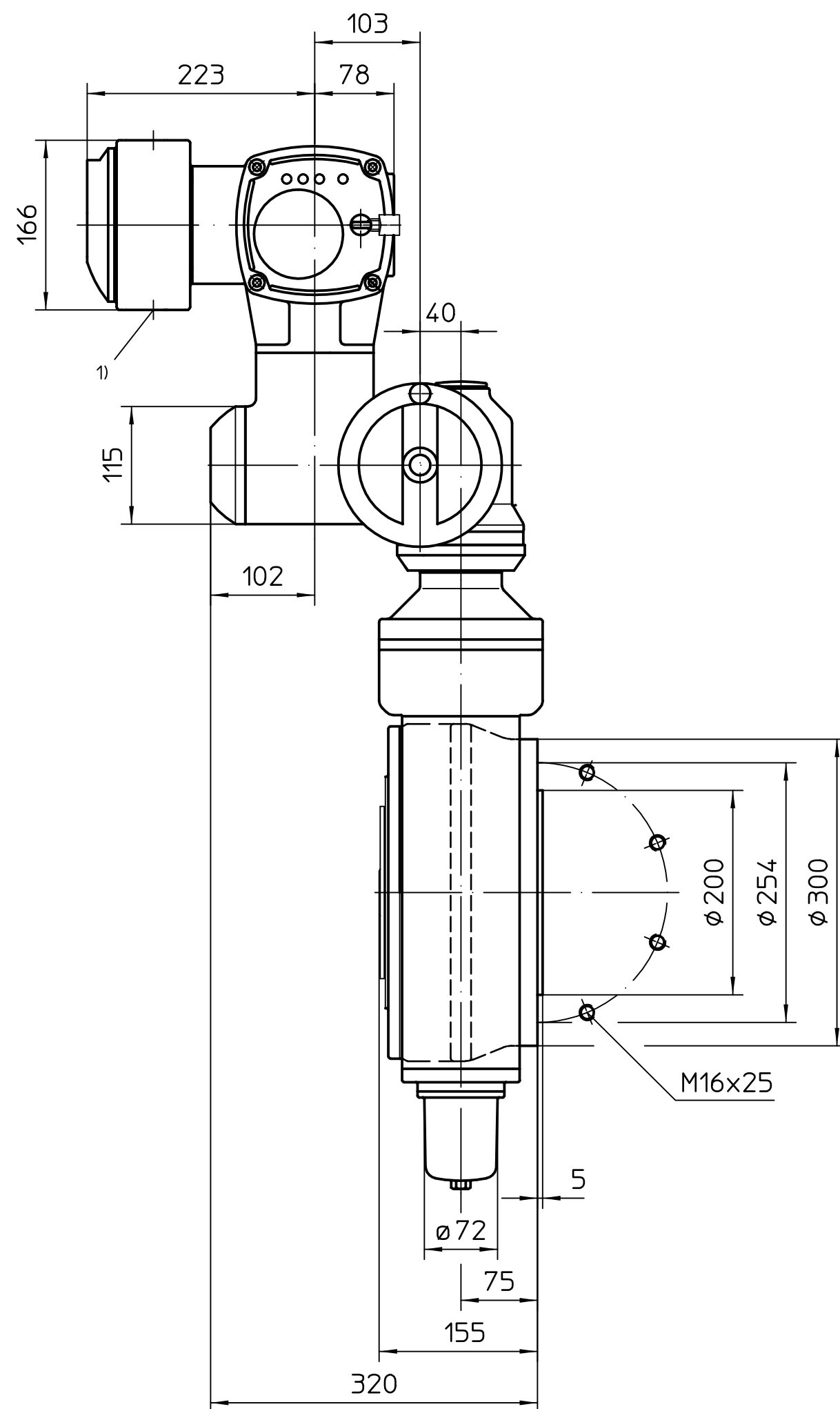
Standard version KT Exe
