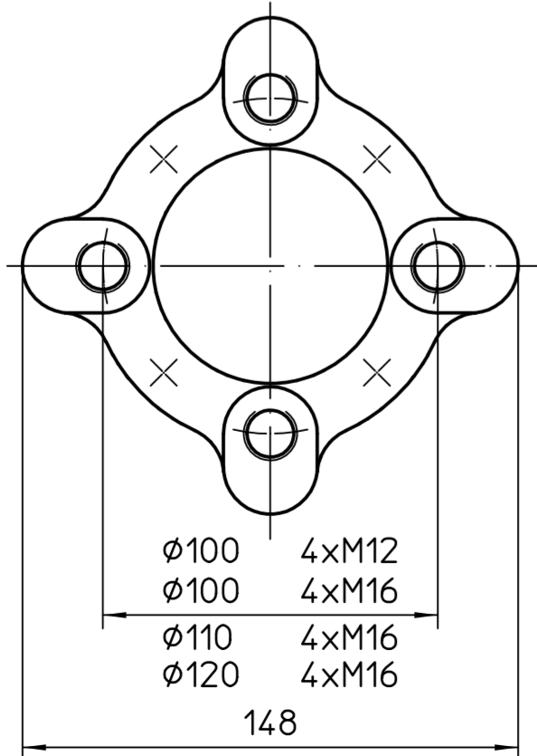
View A connecting ring
