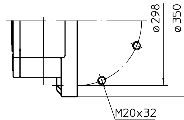
Plane flange option
