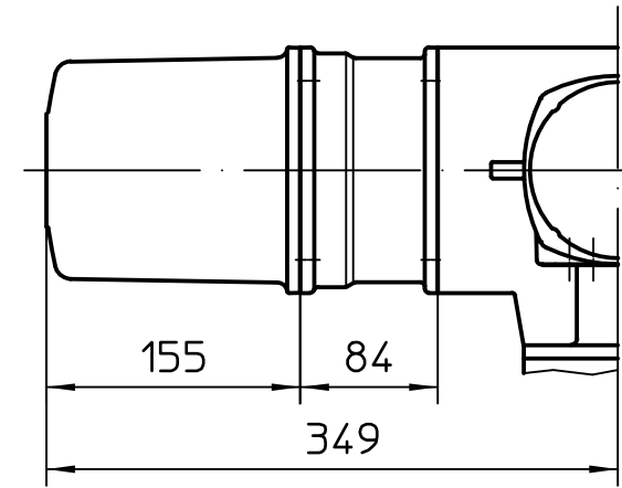
Version with thermal overload relay
