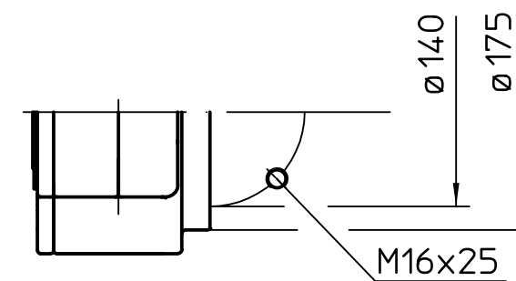
Plane flange option
