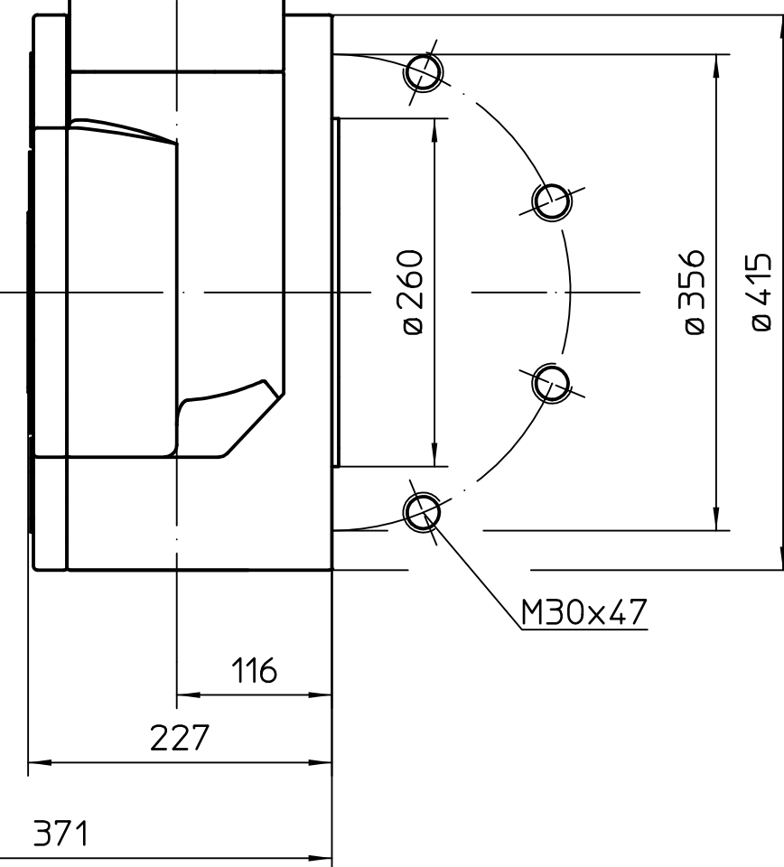
Plane flange option
