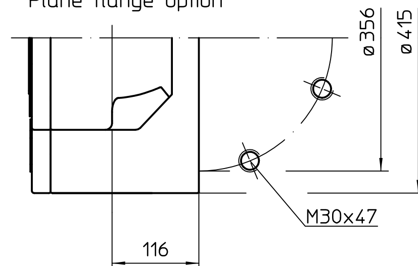
Plane flange option
