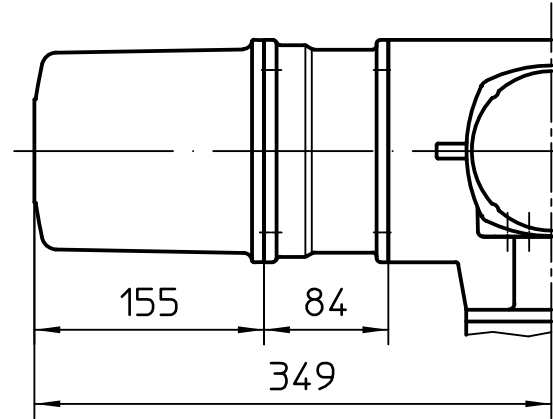
Version with thermal overload relay
