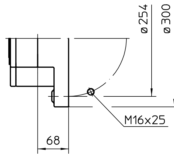
Plane flange option
