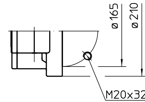
Plane flange option
