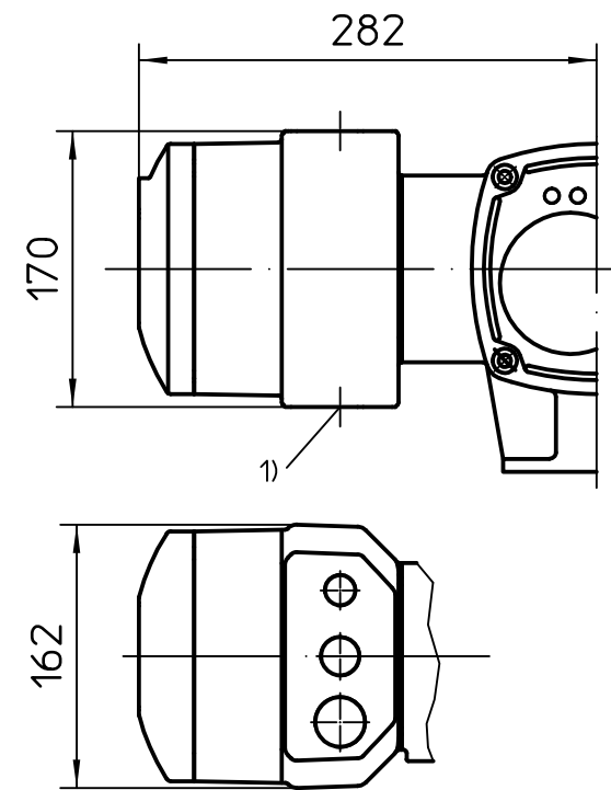
Version KT Exd Version KM Exd
