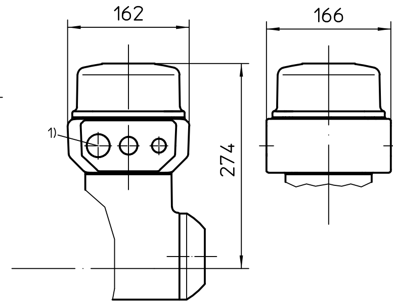
Version KM Exe
