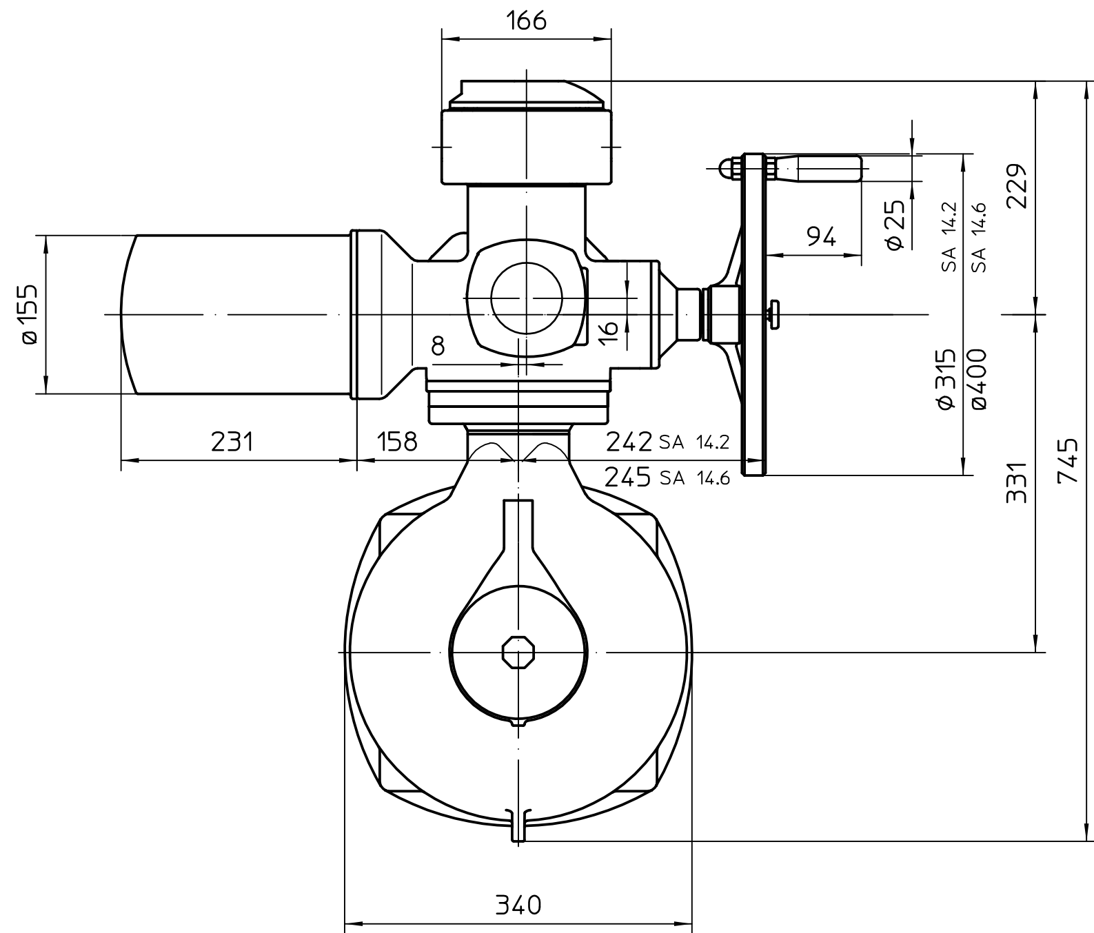
Version standard KT Exe
