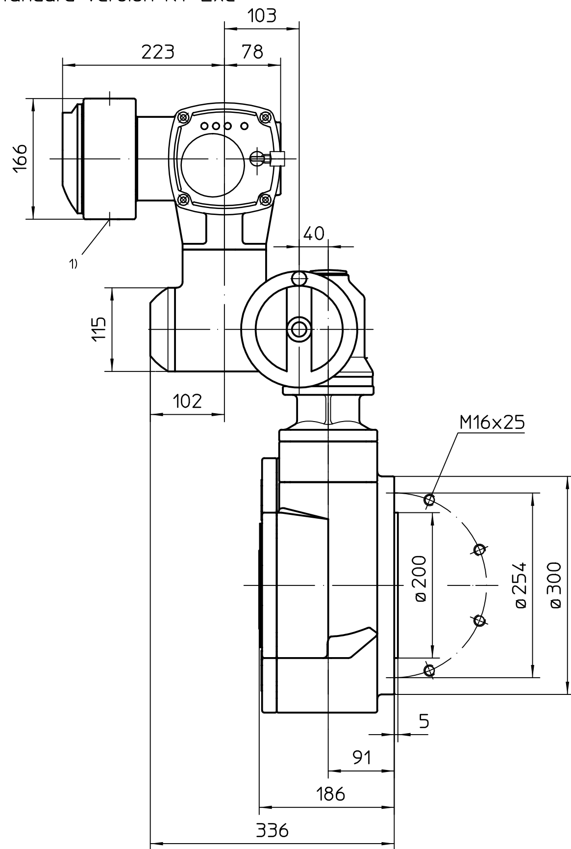
Standard version KT Exe
