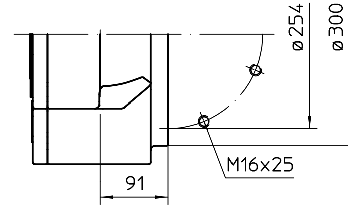
Plane flange option
